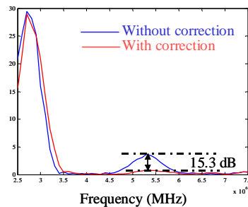
Fig. 4. Spectrum of the backscattered echoes with and without cancellation of the harmonics by time reversal processing.
