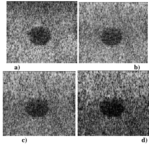
Fig. 8. Experimental harmonic images obtained using distorted emission waveforms. The harmonic content of the agar gelatin phantom surrounding the anechoic inclusion is progressively cancelled.
