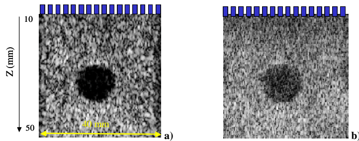
Fig. 6. a) fundamental and b) harmonic image of an Agar gelatin phantom presenting an anechoic inclusion. The contrast in the harmonic image is quite low. M.I. was equal to 1. The probe is working at 4.3 MHz.
