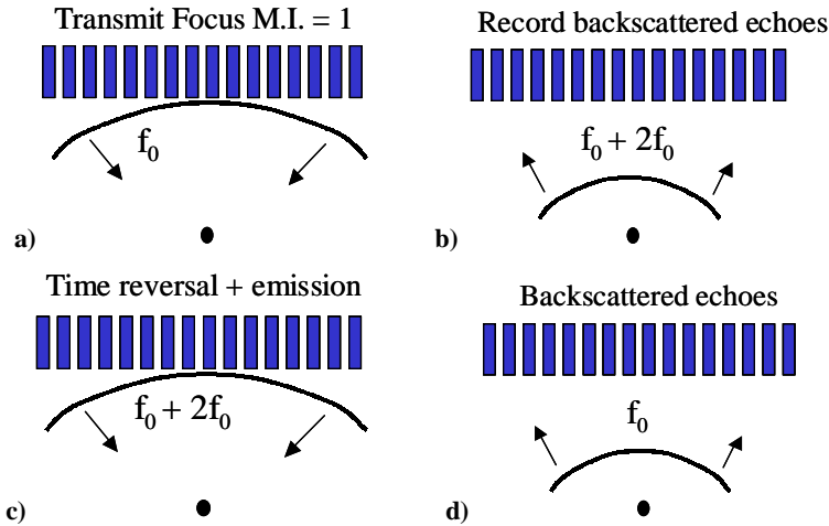
Fig. 2. Principle of the adaptive cancellation of harmonics due to nonlinear propagation.
