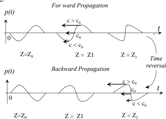
Fig.1. Time reversal invariance in the nonlinear regime.
