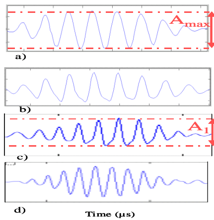
Fig. 3. Experimental results : a) signal emitted by the array; b) backscattered echo after nonlinear propagation in water; c) time reversal and transducer bandwidth correction of the received echo; d) backscattered echo after re-emission of the signal presented in Fig. 3.c.
